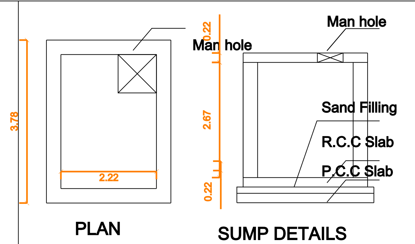
SUMP DETAILS
