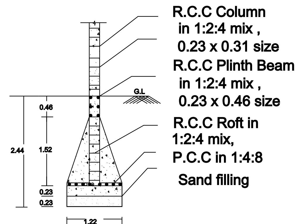
COLUMN DETAILS
