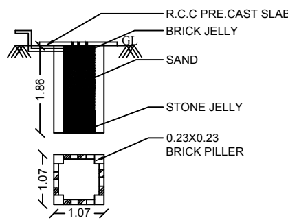
PLAN AND SECTION OF RAINWATER COLLECTION WELL
