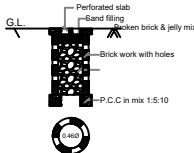
PERCOLATION PIT FOR 30 Sq. m
