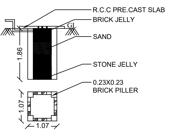
AN AND SECTION OF INWATER COLLECTION ELL
