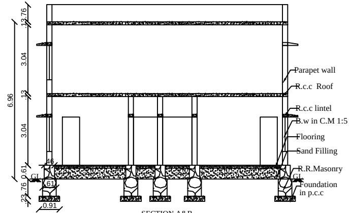
SECTION A&B
