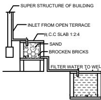
DETAILS OF FILTER BED & WELL NTS
