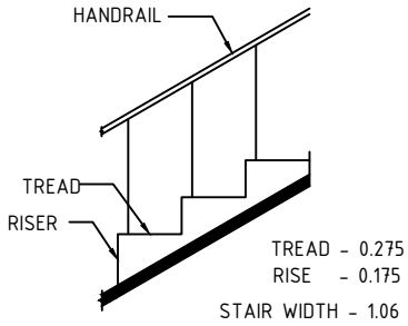
STAIRCASE DETAILS NTS
