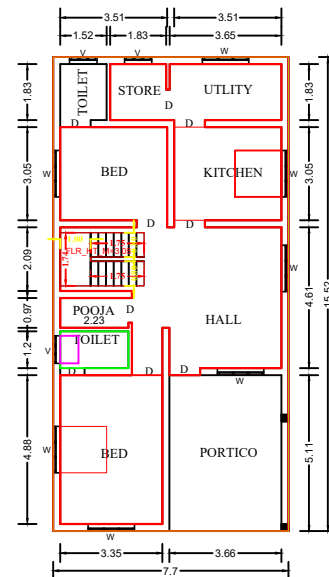
G.FLOOR PLAN
