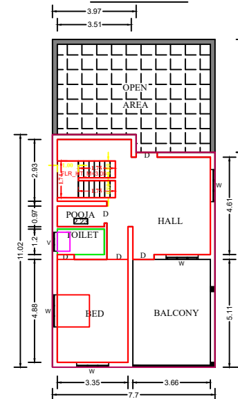
F.FLOOR PLAN
