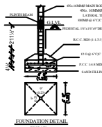
FOUNDATION DETAILS
