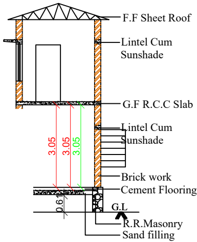
CROSS SECTION ON A-A
