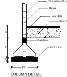
COLUMN DETAIL
