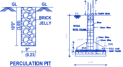
FOUNDATION DETAILS SCALE : 1:50.
