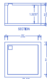
DETAILS OF COLLECTION SUMP FOR RAIN WATER HARVESTING OF ROOF TOP RAIN WATER RWV_CAPACITY_L=5000LTRS
