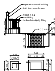
Sump and Filter Bed
