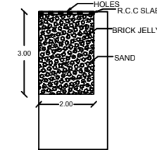
SECTION OF RAIN WATER COLLECTING TANK
