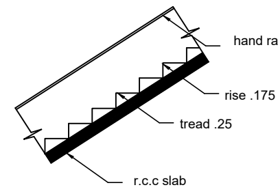
STAIR
