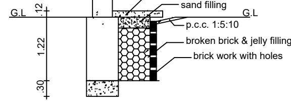
PLINTH BOUNDARY PERCOLATION PIT
