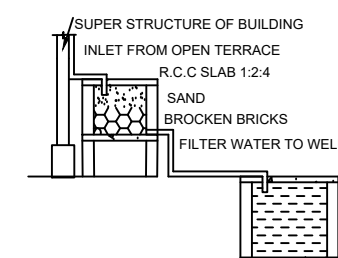
RAINWATER HARVESTING
