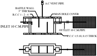
SEPTIC TANK & TRENCH
