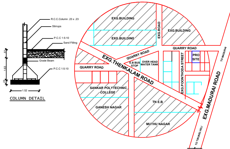
TOPO PLAN ( As On Site ) NOT TO SCALE
