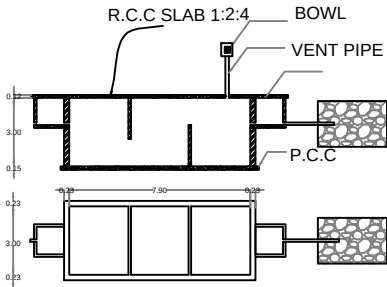
SEPTIC TANK AND TRENCH NTS
