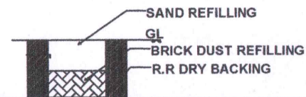
DETAILS OF RAIN WATER HARVESTING
