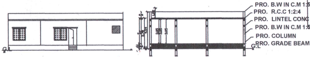
SECTION ON A A
