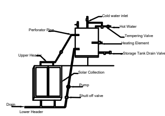
Details of Solar Water Heater (NTS)
