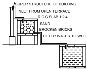
RAINWATER HARVESTING
