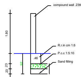
Compound wall Detail SCALE : (1:50)
