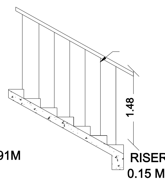
STAIRCASE DETAILS
