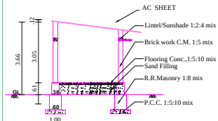
SECTION ON C-D
