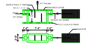
Septic tank and trench
