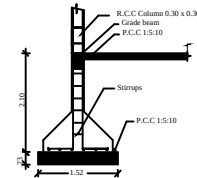
Column Detail
