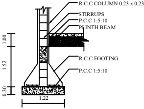
COLUMN DETAILS
