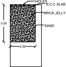
SECTION OF RAIN WATER COLLECTING TANK
