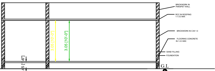
SECTION AB
