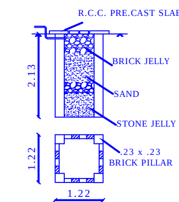
PLAN & SECTION OF RAIN WATER COLLECTION WELL
