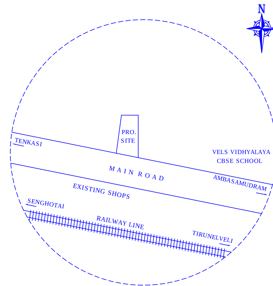
TOPO PLAN
