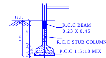
RCC COLUMN FOUNDATION DETAILS
