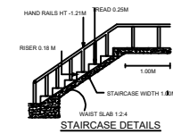
STAIRCASE DETAILS
