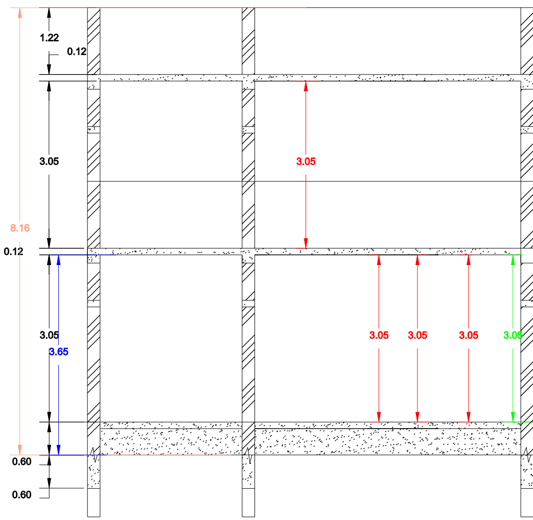
SECTION"AA"
