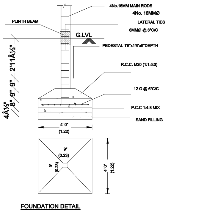
FOUNDATION DETAIL
