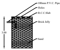
SECTION OF RAIN WATER COLLECTING TANK
