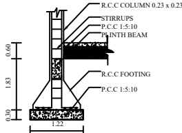
COLUMN DETAILS
