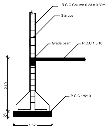
COLUMN DETAIL
