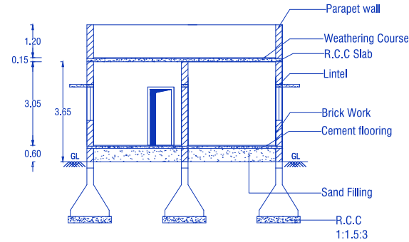
CROSS SECTION ON 'AB'
