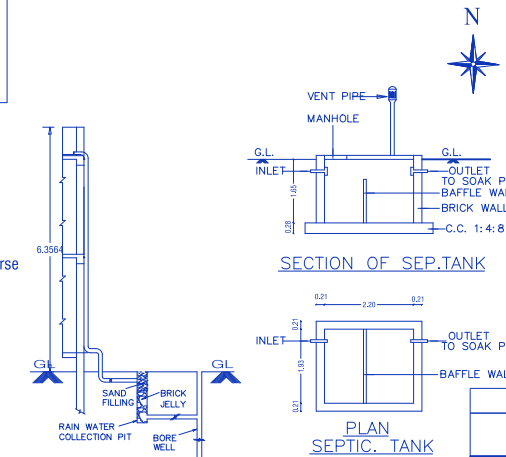
RAIN WATER HARVESTING SYSTEM RWH_CAPACITY_L=1000LTRS
