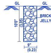
PERCOLATION PIT
