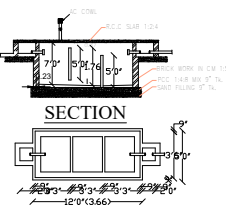
SECTION PLAN SEPTIC TANK DETAILS
