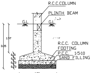
FOUNDATION DETAIL
