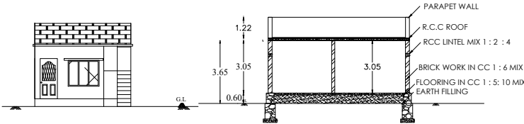
SECTION ON AB & ( HALF ELEVATION)
