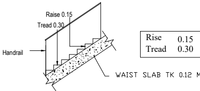
STAIRCASE DETAIL
