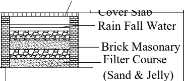
PLAN SECTION OF RECHARGE TRENCH METHOD
