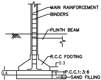
TYPICAL SECTION OF R.C.C COLUMN FOUNDATION
