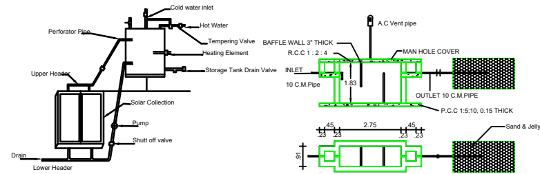
Details of Solar Water Heater (NTS)
