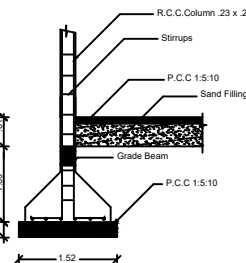
COLUMN DETAIL
