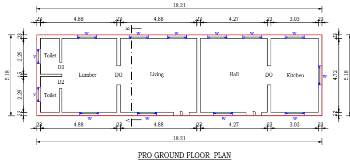
PRO GROUND FLOOR PLAN
