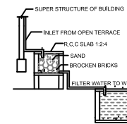
DETAILS OF FILTER BED & WELL
