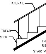
STAIRCASE DETAILS
