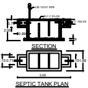
SEPTIC TANK PLAN
