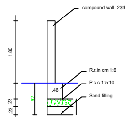
Compound wall Detail SCALE : (1:50)
