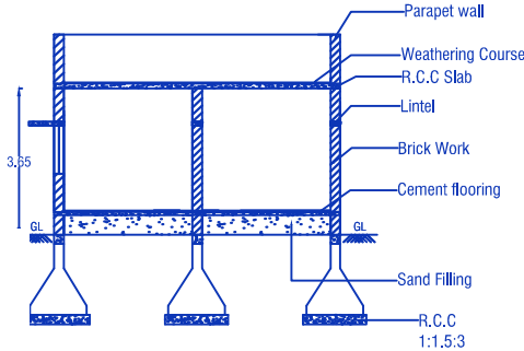
CROSS SECTION ON 'A-B'
