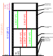
SECTION ON AA
