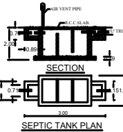
SEPTIC TANK PLAN
