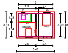
GROND FLOOR PLAN
