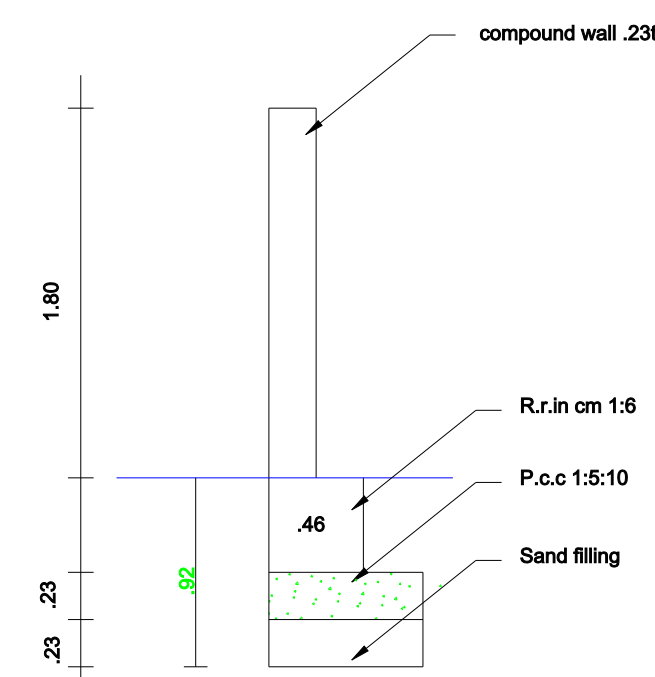
Compound Wall Detail SCALE : (1:50)
