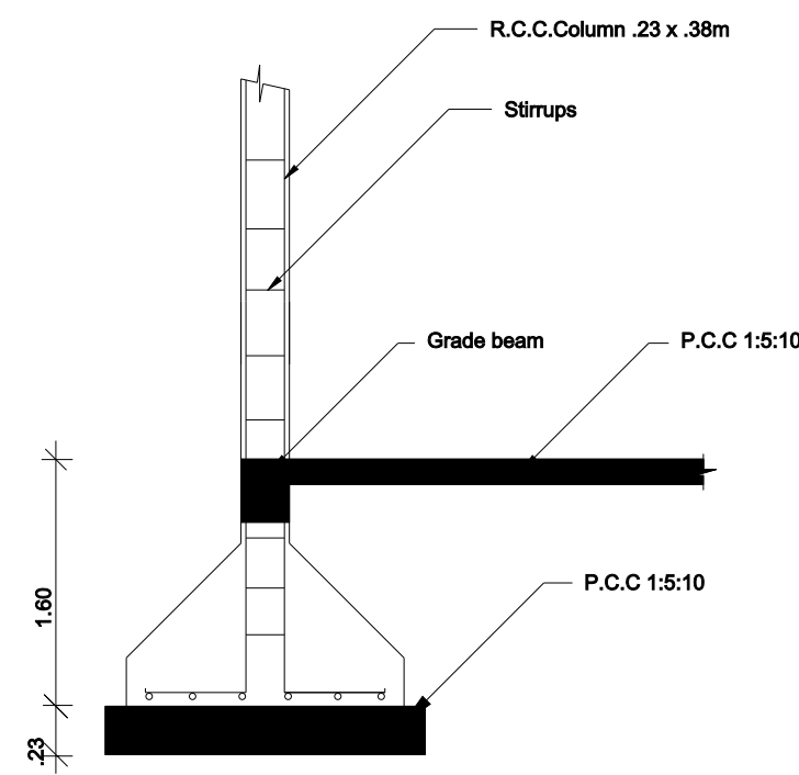
COLUMN DETAIL
