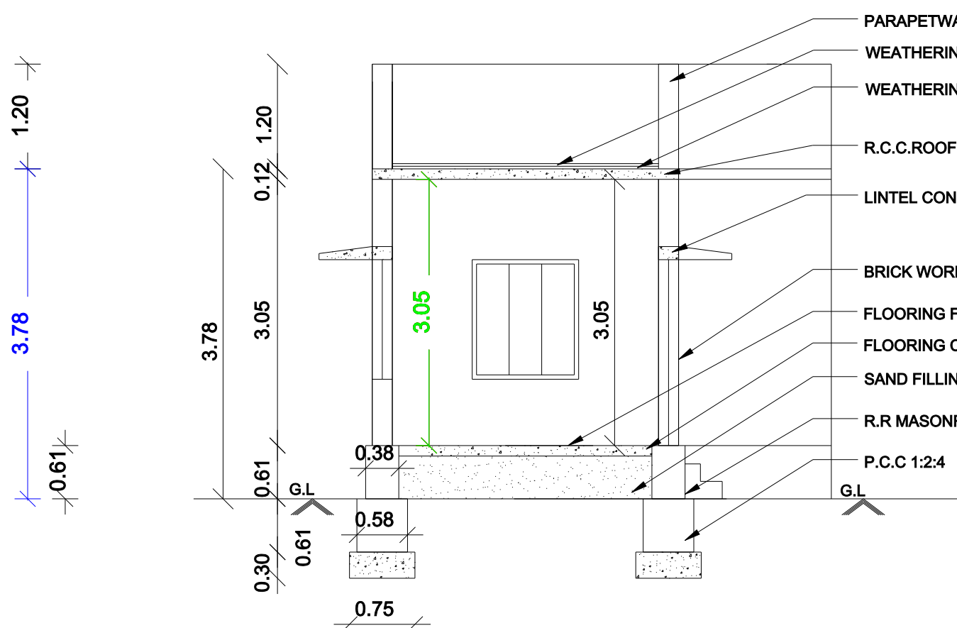
SECTION AT A-B
