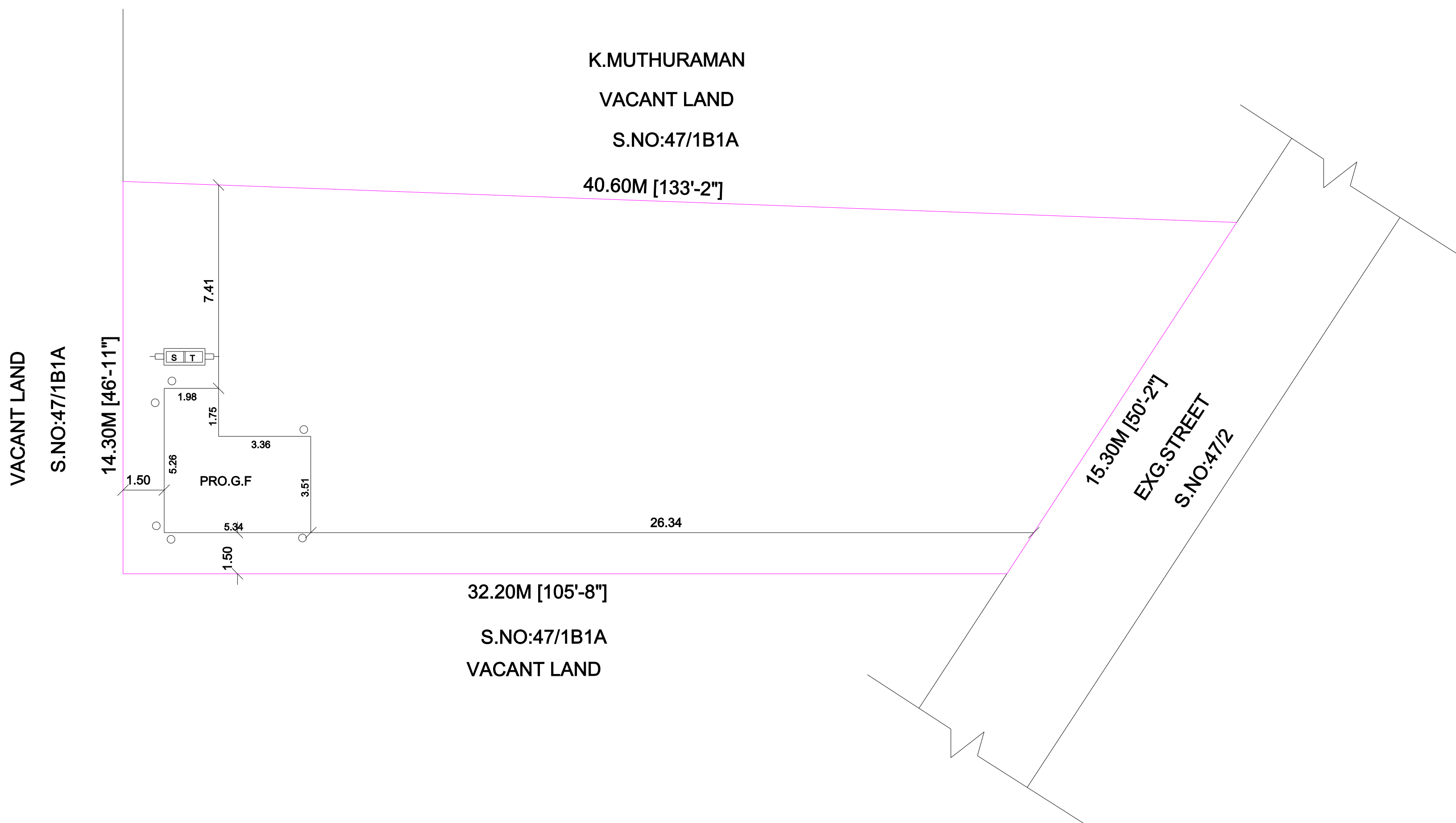
SITE PLAN
