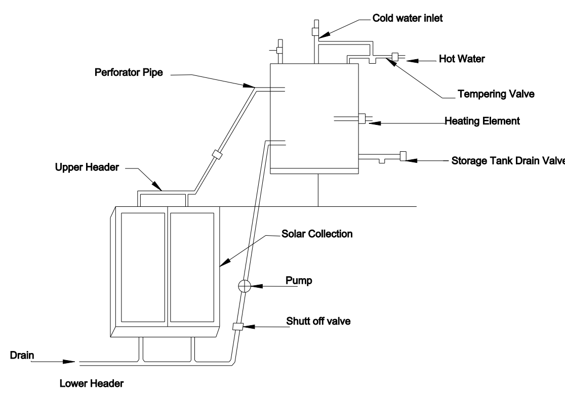
Details Of Solar Water Heater (NTS)
