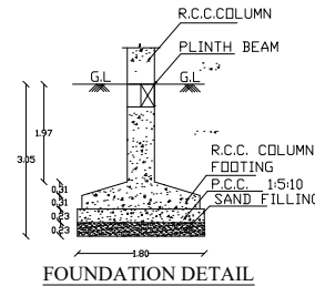
FOUNDATION DETAIL
