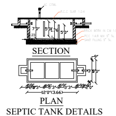
PLAN SEPTIC TANK DETAILS
