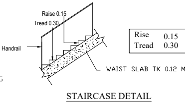
STAIRCASE DETAIL
