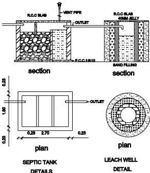
1000 GALLONS CAPACITY SEPTIC TANK (NTS)
