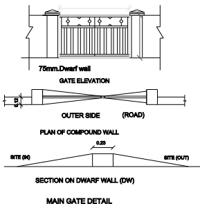
MAIN GATE DETAIL
