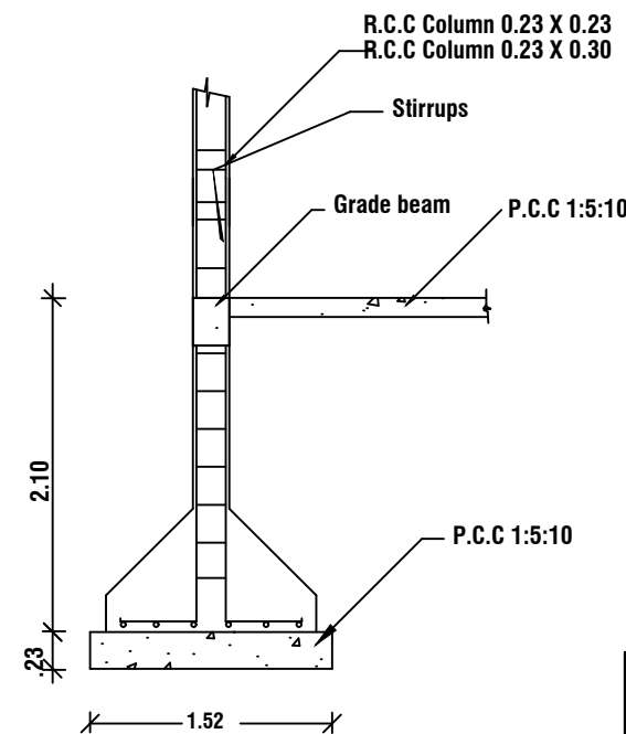
COLUMN DETAIL
