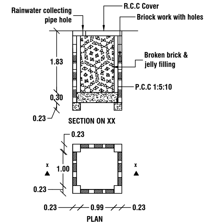
RAINWATER HARVEST WELL
