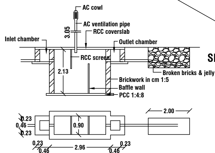
SEPTICTANK DETAILS
