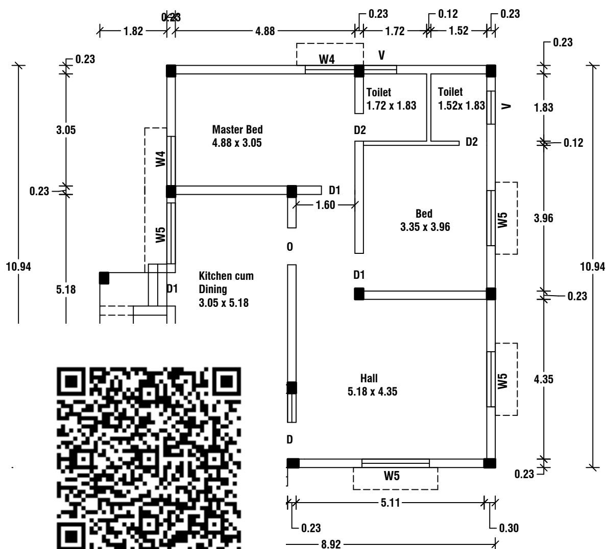
PLAN SCALE 1:100
