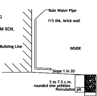
PERCOLATION PIT
