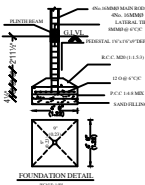
FOUNDATION DETAIL
