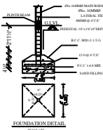
FOUNDATION DETAIL
