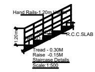
Hand Rails-1.20m Tread - 0.30m Rise - 0.15m Staircase Details Scale:1:500
